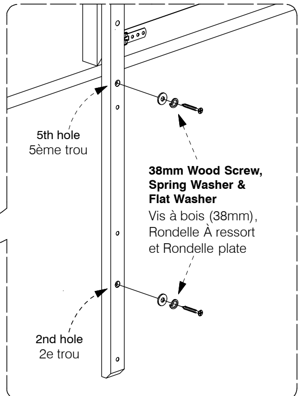
Back of Mirror Dos du miroir
