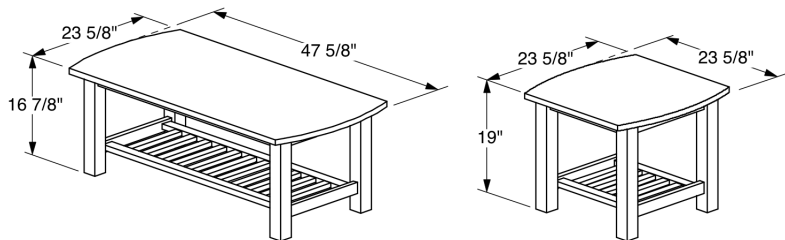
Corona Coffee Table
