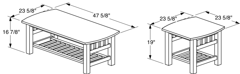
Raleigh Coffee Table
