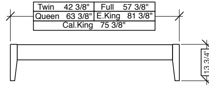
BASIC FOOTBOARD
