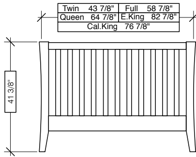
NUTMEG HEADBOARD
