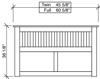
HEADBOARD / FOOTBOARD
