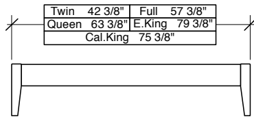
BASIC FOOTBOARD
